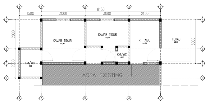
DETAIL DENAH LANTAI I SKALA 1:100
